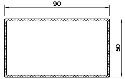
AL. KUTU PR. ( 50 X 90 ) 6099.159
