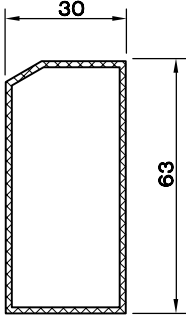
AL. KAPI DESTEK PR. 6145.111
